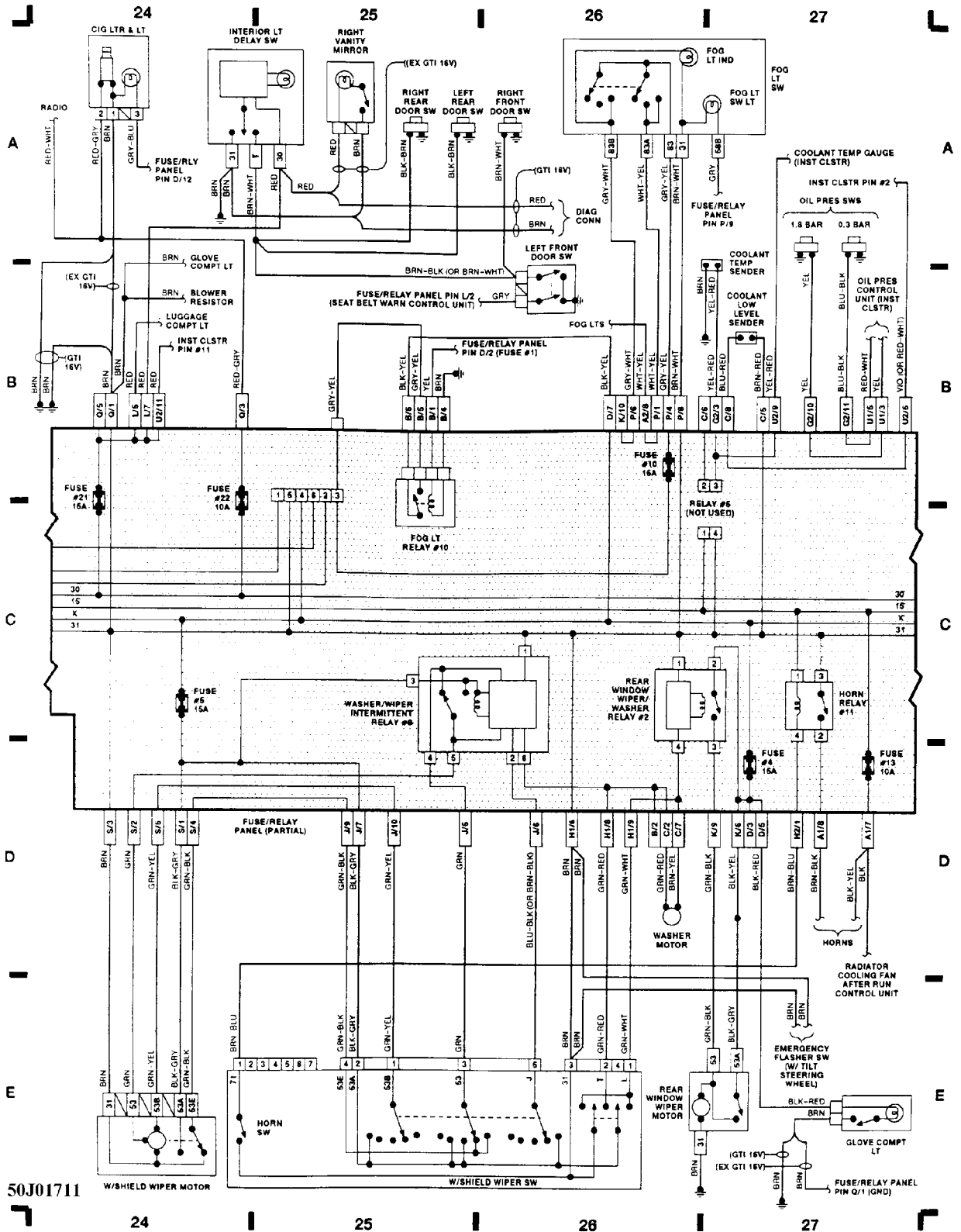
Fig. 7: Fuse/Relay Panel (3 of 4), (Grid 24-27)
